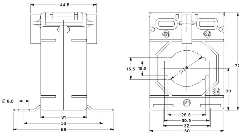
RISH XMER 50/30 (30)
