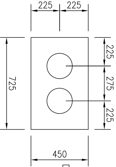
DUCT BANK 200 mm HDPE pipe
