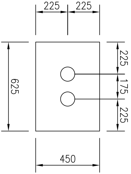
DUCT BANK 100 mm PVC pipe
