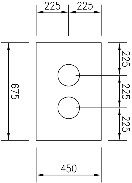
DUCT BANK 150 mm PVC pipe
