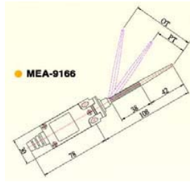
MEA-9166 Plastic mini limit switch, MEA-9166G Plastic mini limit switch, flat tail
