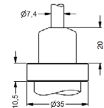
cable outlet, cable with ventilation tube (IP 68) 6
